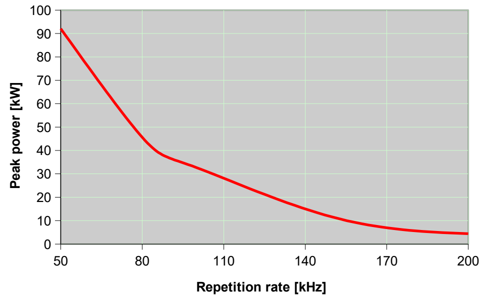
Wedge XF 532nm Plus: Peak Power
